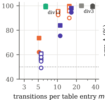
(b) per-step q and accuracy vs. m
