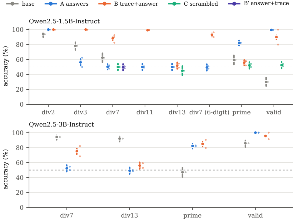
Figure 2: Accuracy by arm and task at n = 180 , pooled over seeds with 95% Wilson intervals (240 test items per task and seed); small dots are single seeds; one row per model with at least three tasks (0.5B and 7B are in Table 4). Dashed line: majority class.
