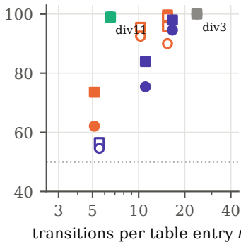
(b) per-step p and accuracy vs. m
