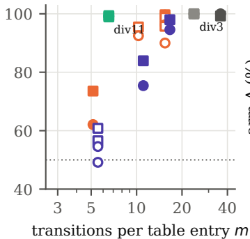
(b) per-step p and accuracy vs. m
