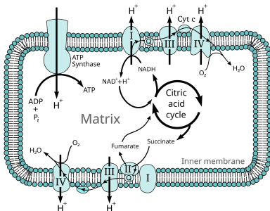
Mitochondrial Electron Transport Chain
