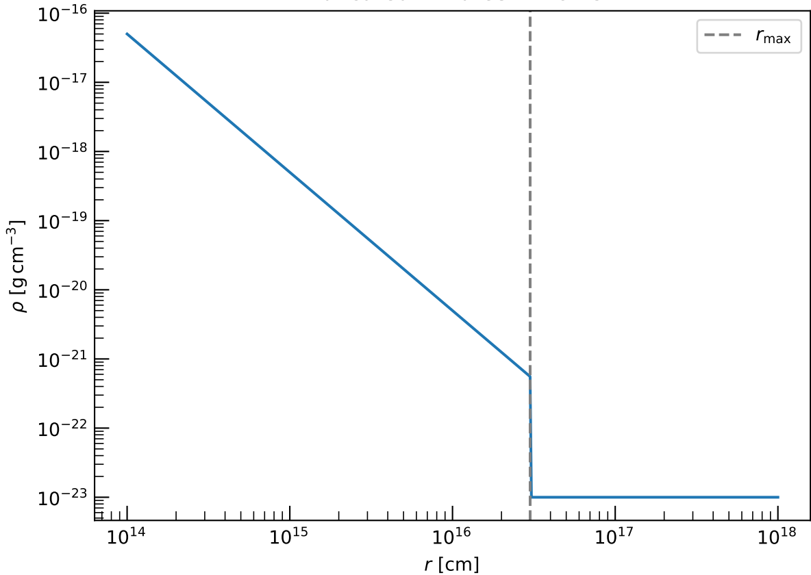
Truncated Wind CSM Profile
