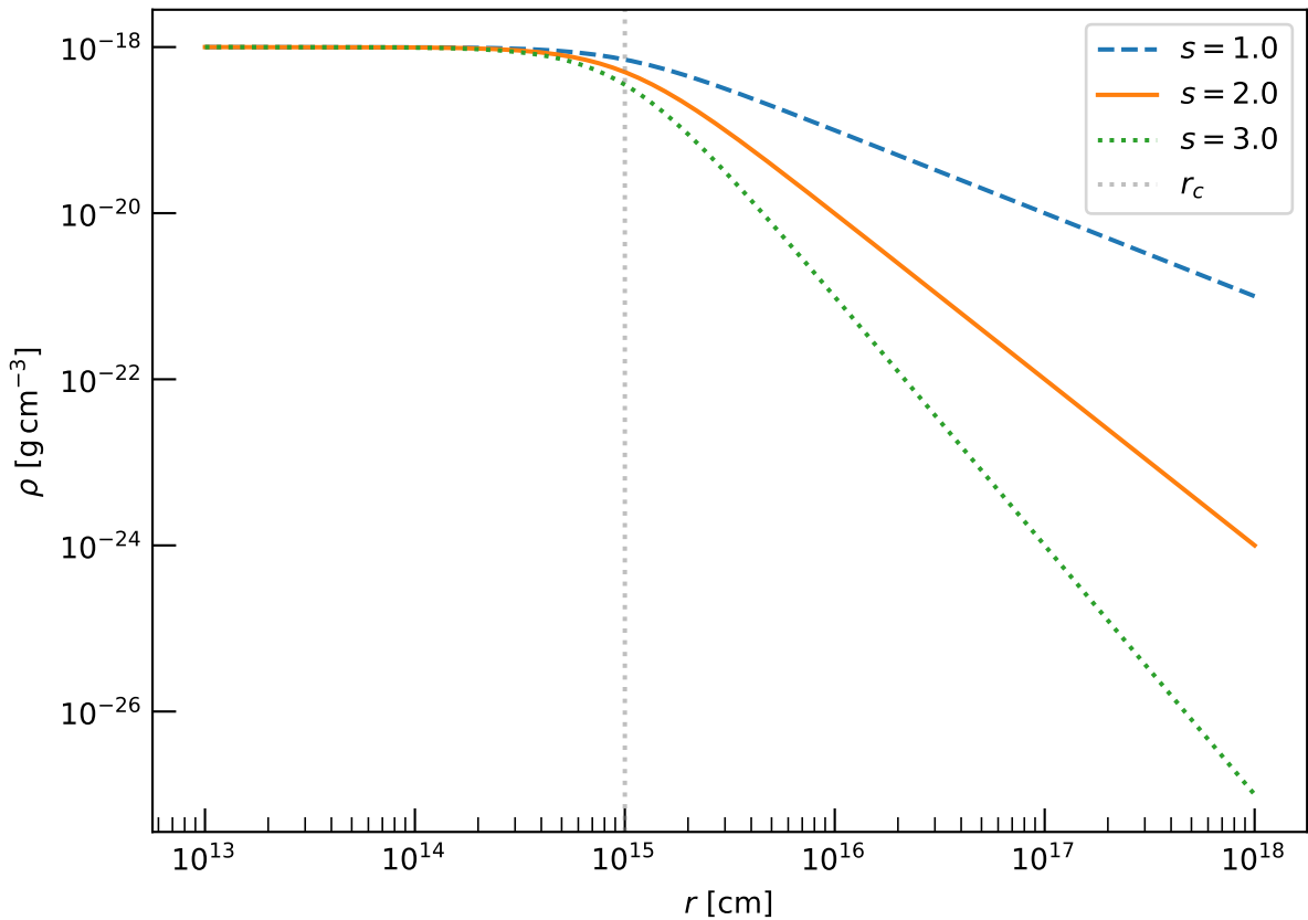
Cored Power-Law CSM Profile
