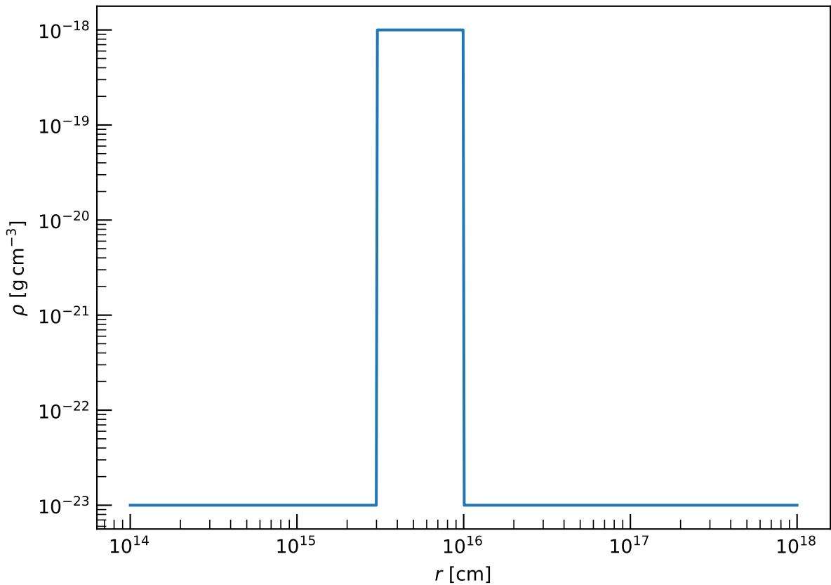
Top-Hat Shell CSM Profile
