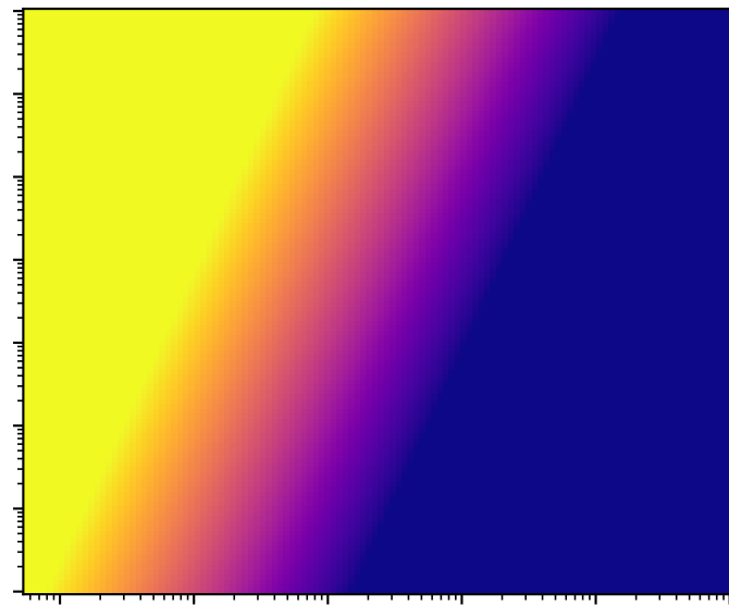
Kramers (analytic)
