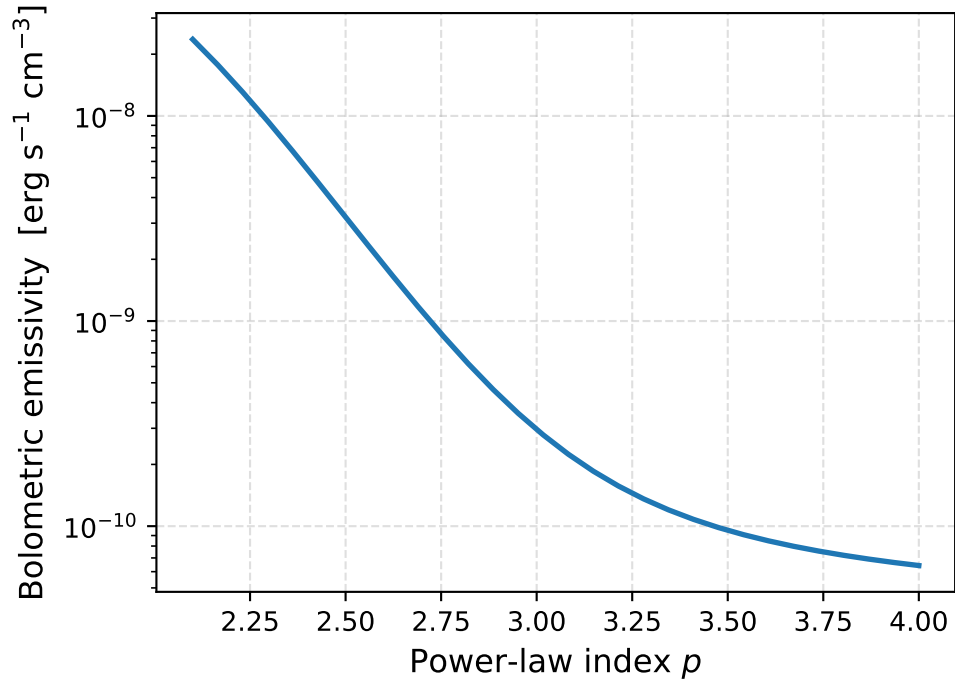
Power-law distribution
