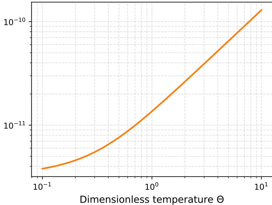
Maxwell-Jüttner distribution
