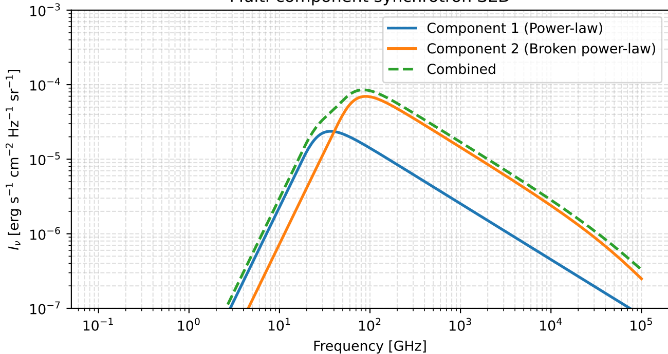
Multi-component synchrotron SED
