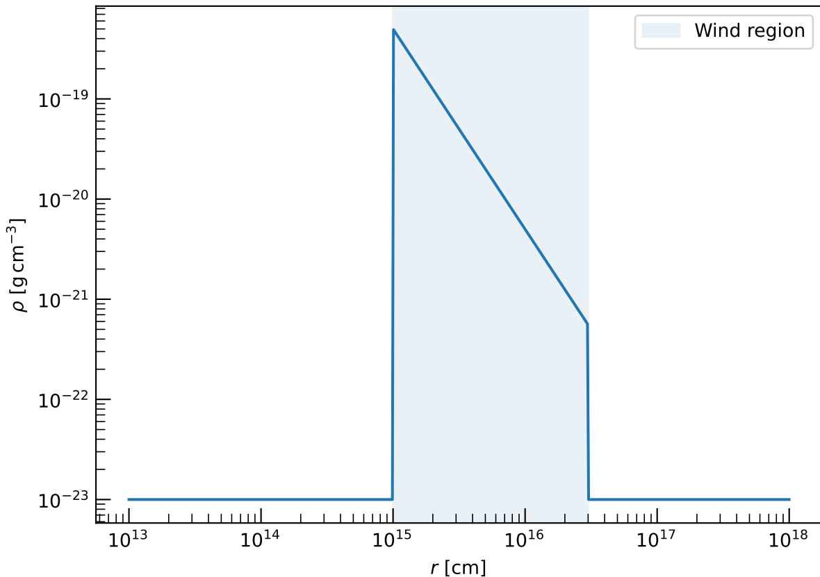
Finite Wind CSM Profile
