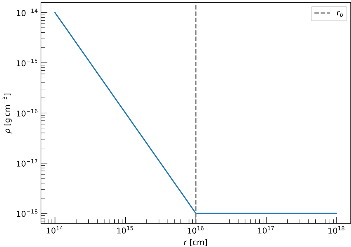
Broken Power-Law CSM Profile
