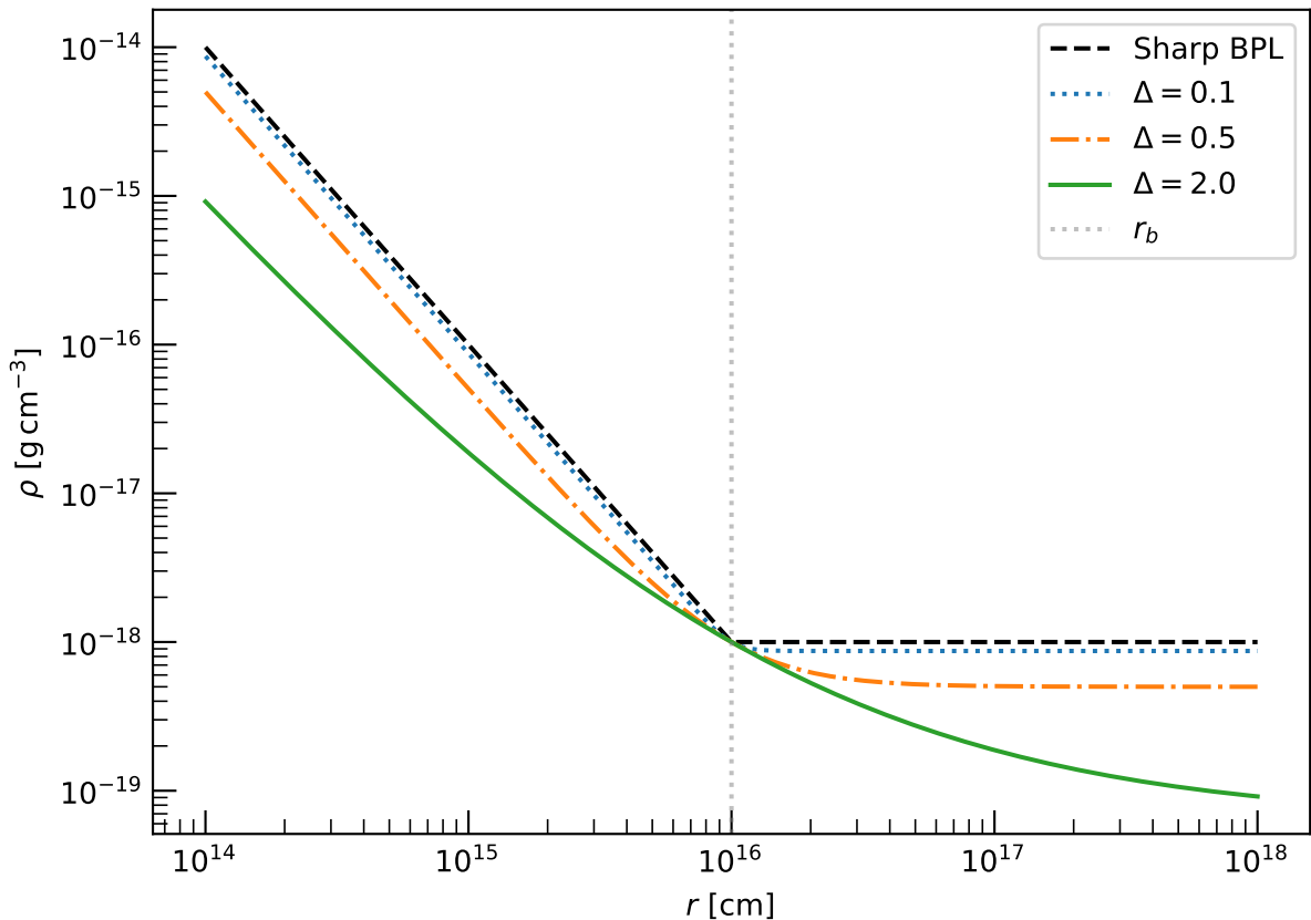
Smooth Broken Power-Law CSM Profile
