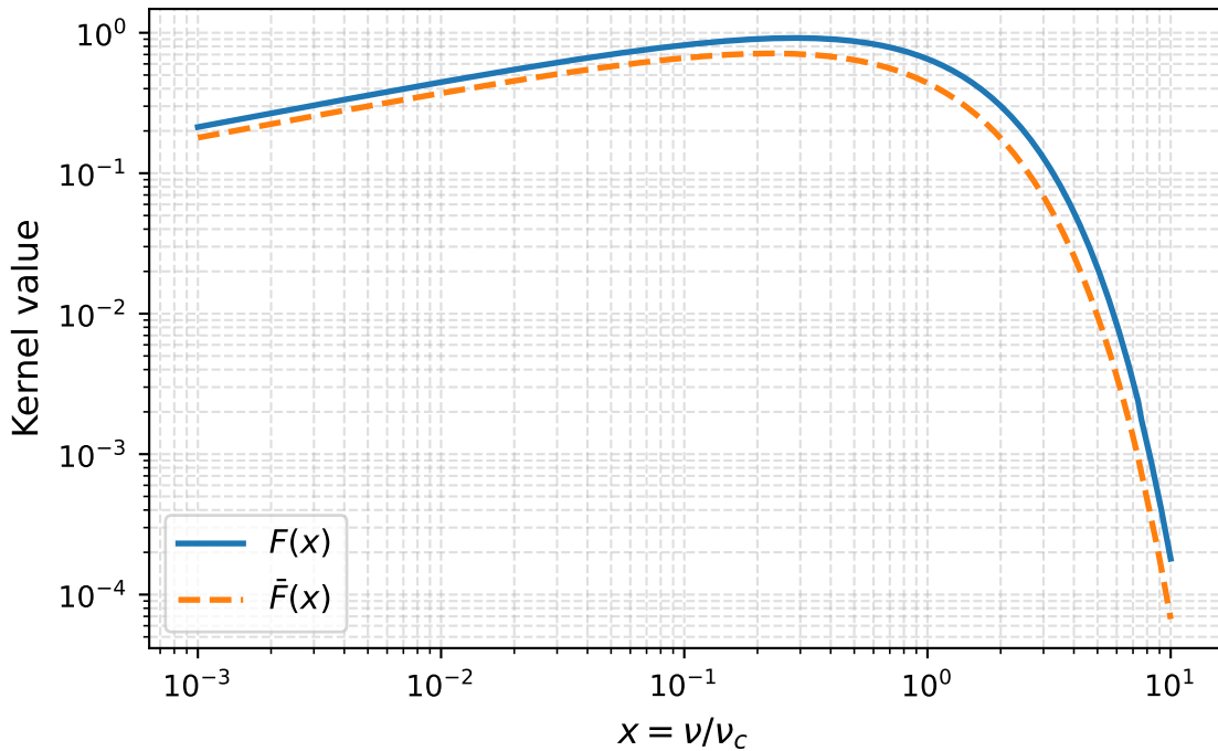
Synchrotron kernel functions
