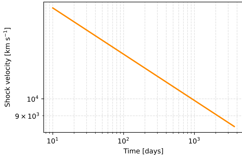
Shock Velocity
