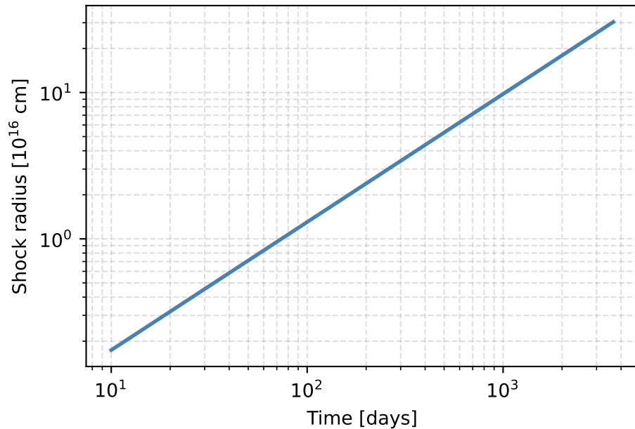
Shock Radius
