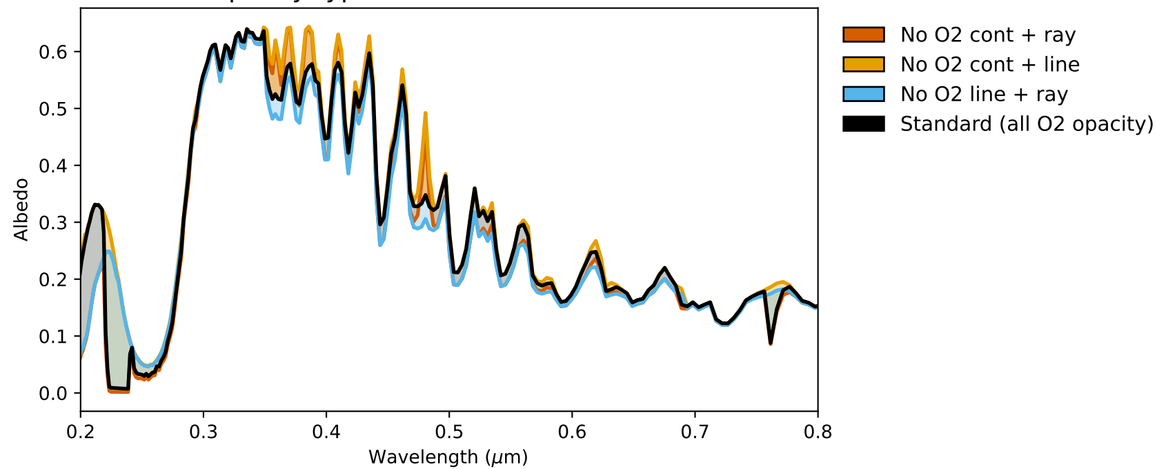
c. Two O2 opacity types excluded
