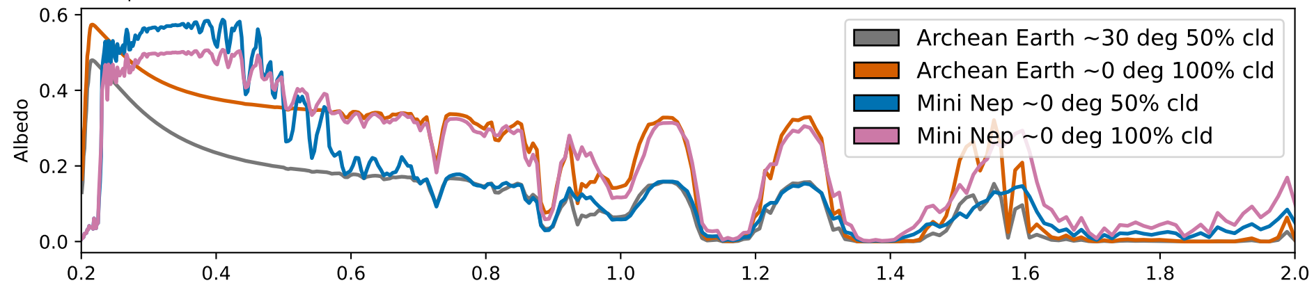
c. Improved Fits based on Cloud/Phase
