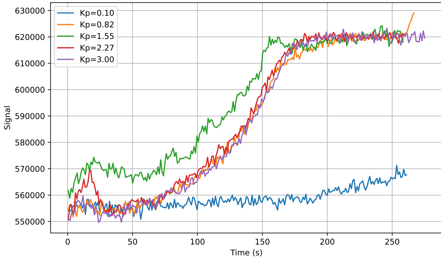
Signal vs Time (Kp sweep)
