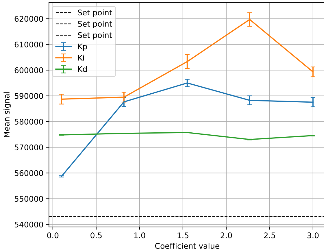
Mean Signal vs PID Coefficient
