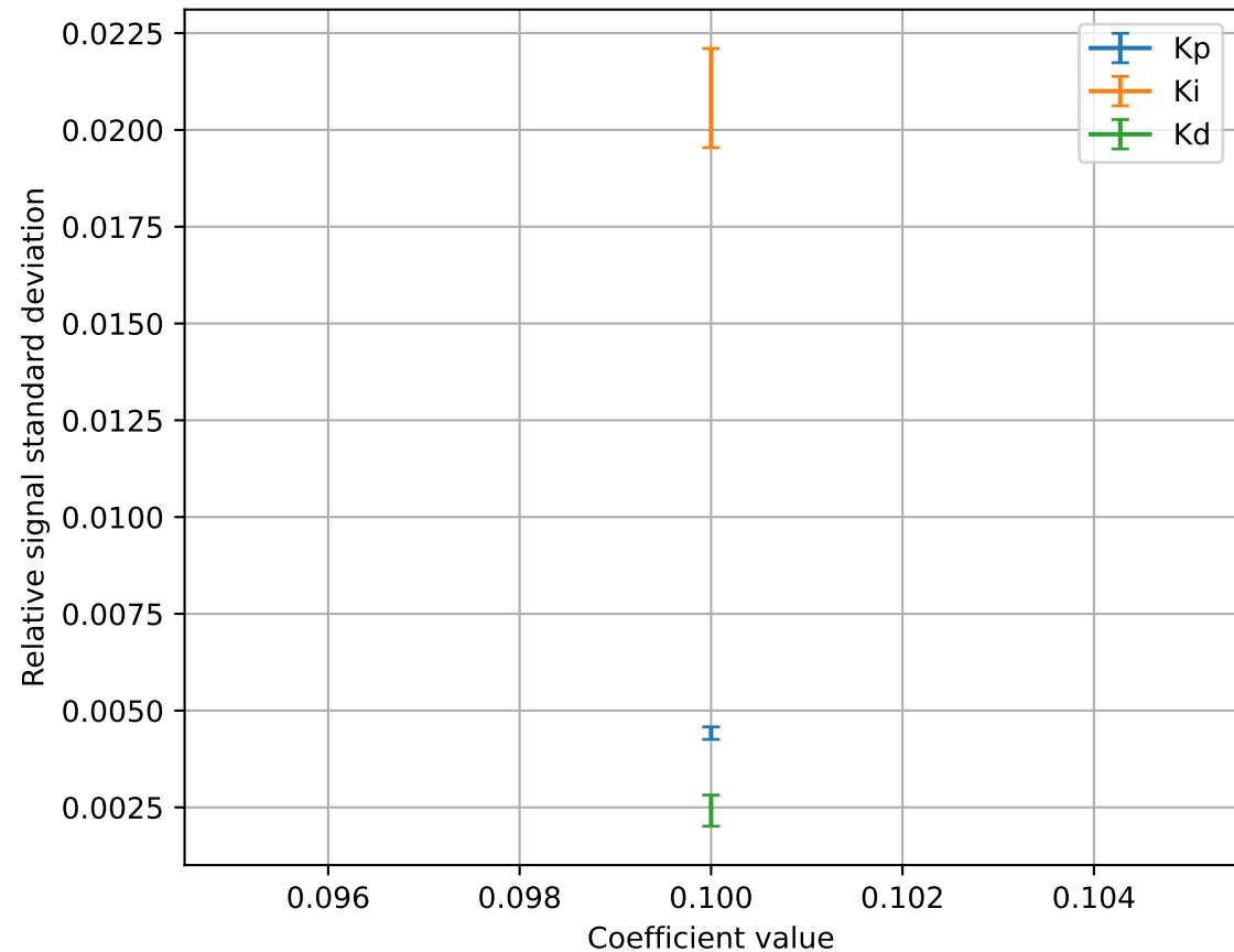
Relative Signal Std Dev vs PID Coefficient
