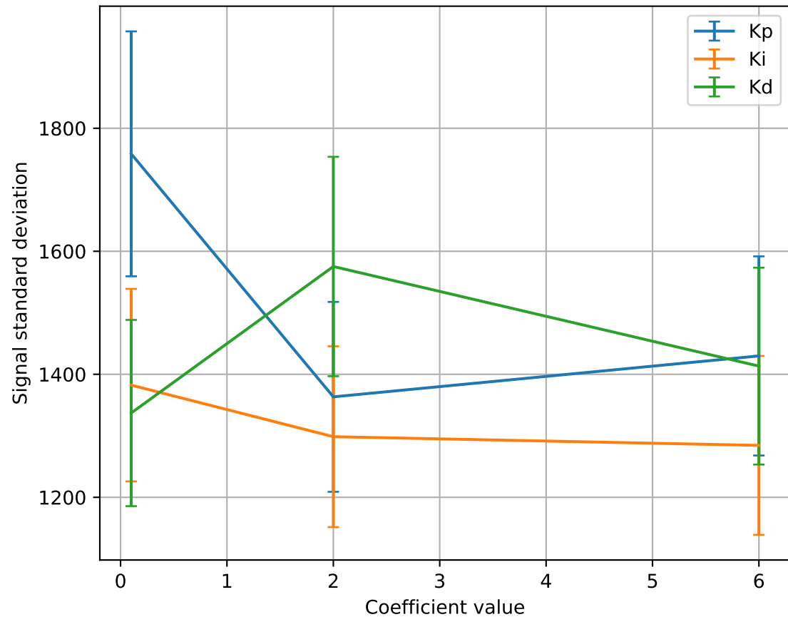
Signal Std Dev vs PID Coefficient
