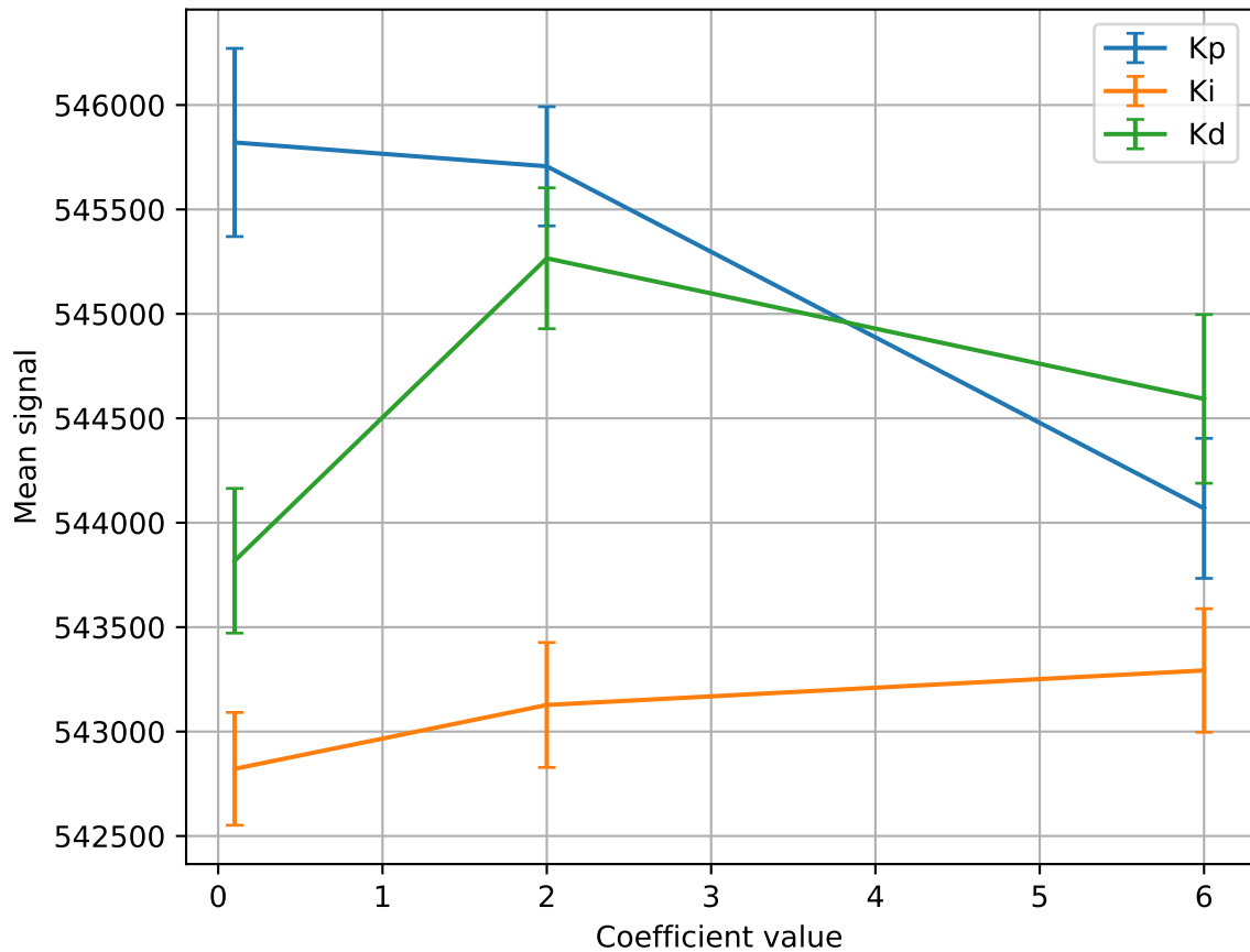
Mean Signal vs PID Coefficient
