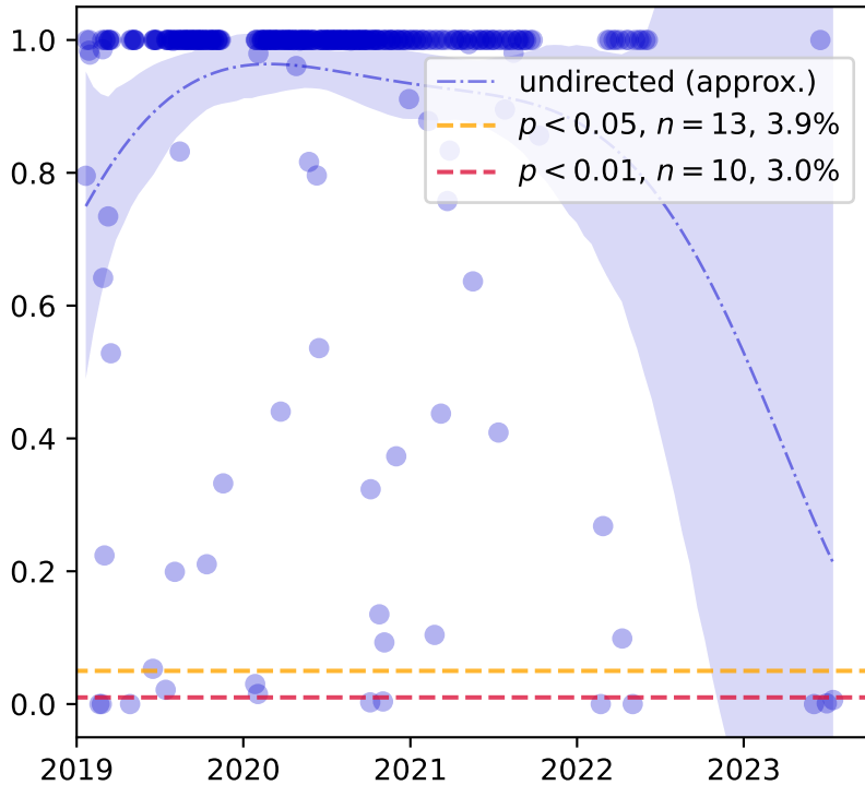
Kolmogorov-Smirnov test p -value (degree distribution)
