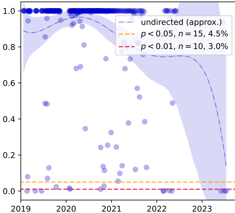
Kolmogorov-Smirnov test p -value (shared node capacity distribution)
