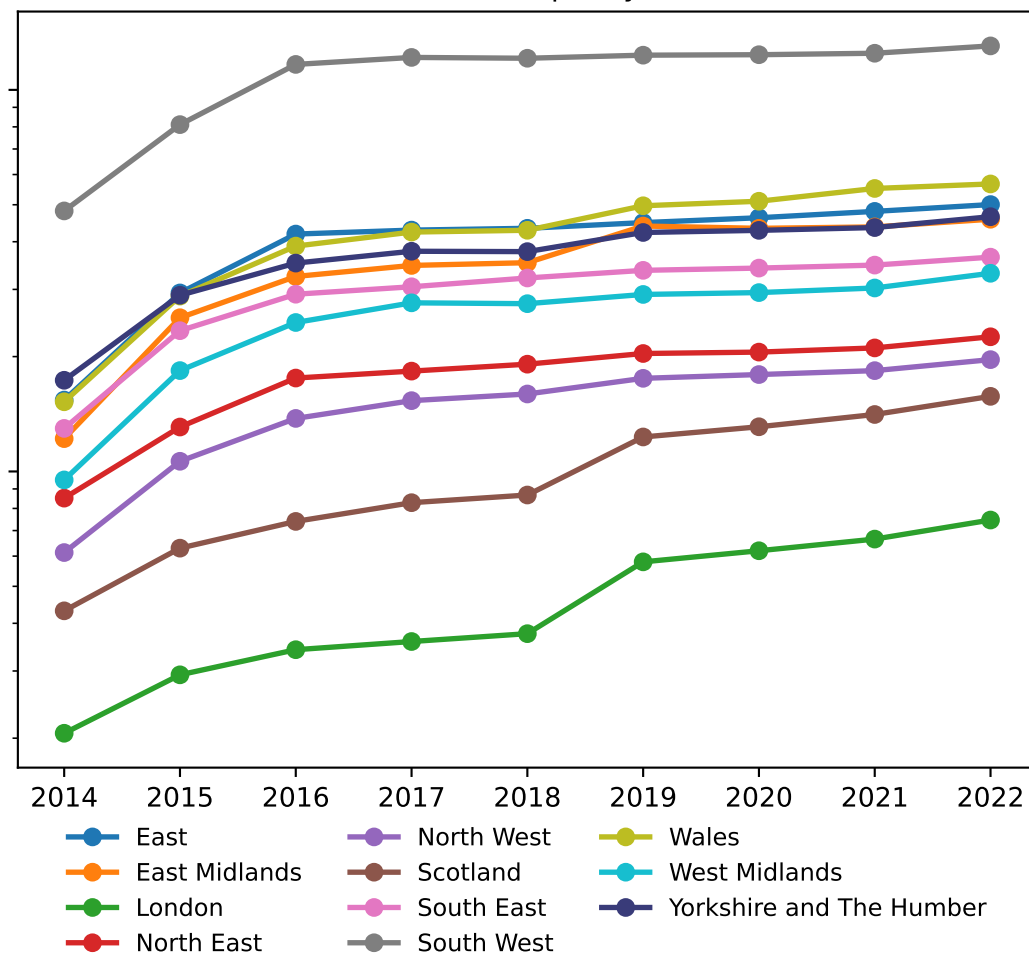
PV installed capacity [kW]
