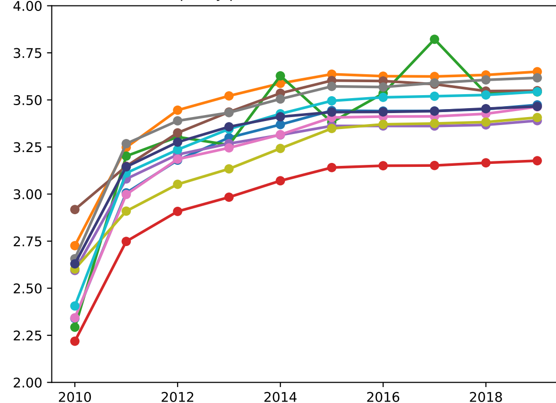
PV capacity per installation [kW / installation]
