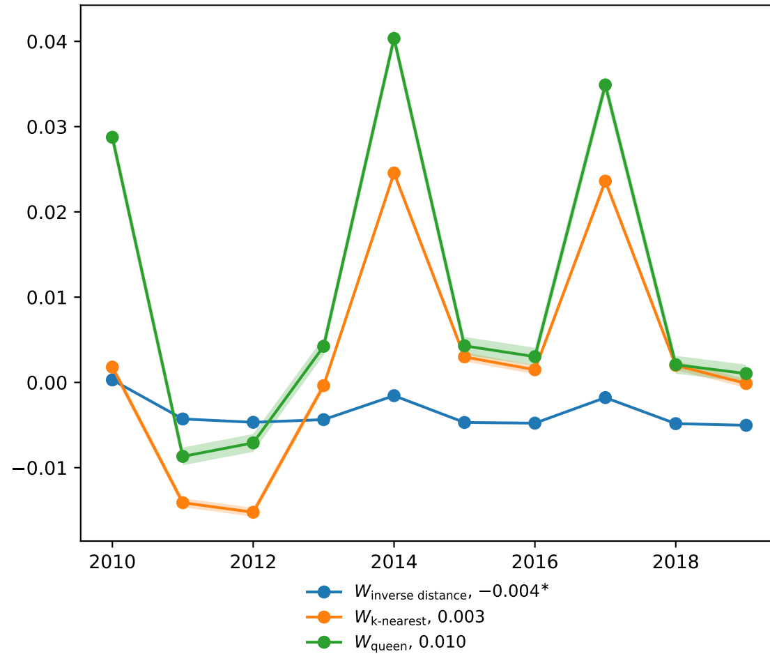
PV installations
