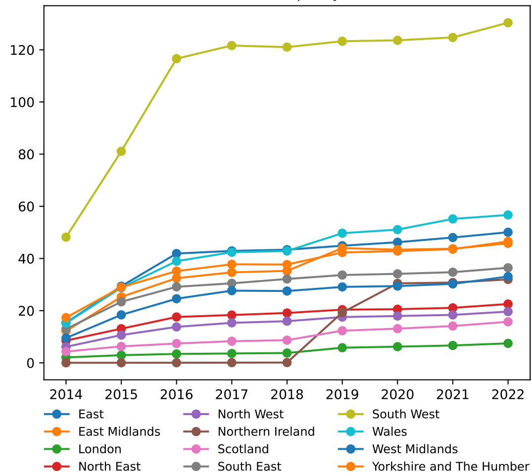
PV installed capacity [MW]
