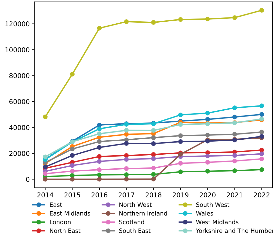
PV installed capacity [MW]
