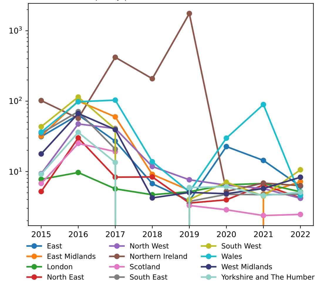
PV capacity per installation [MW / installation]
