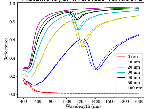
Metallic layer thickness variations
