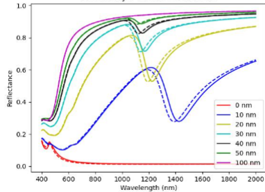
Metallic layer thickness variations
