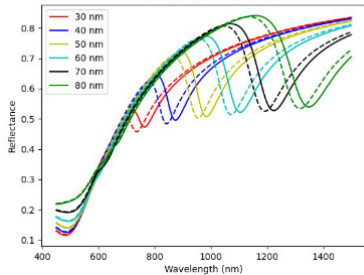
Cube thickness variations
