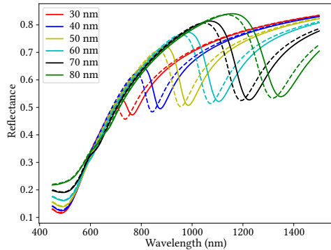
Cube thickness variations
