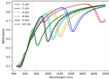
Gap layer thickness variations
