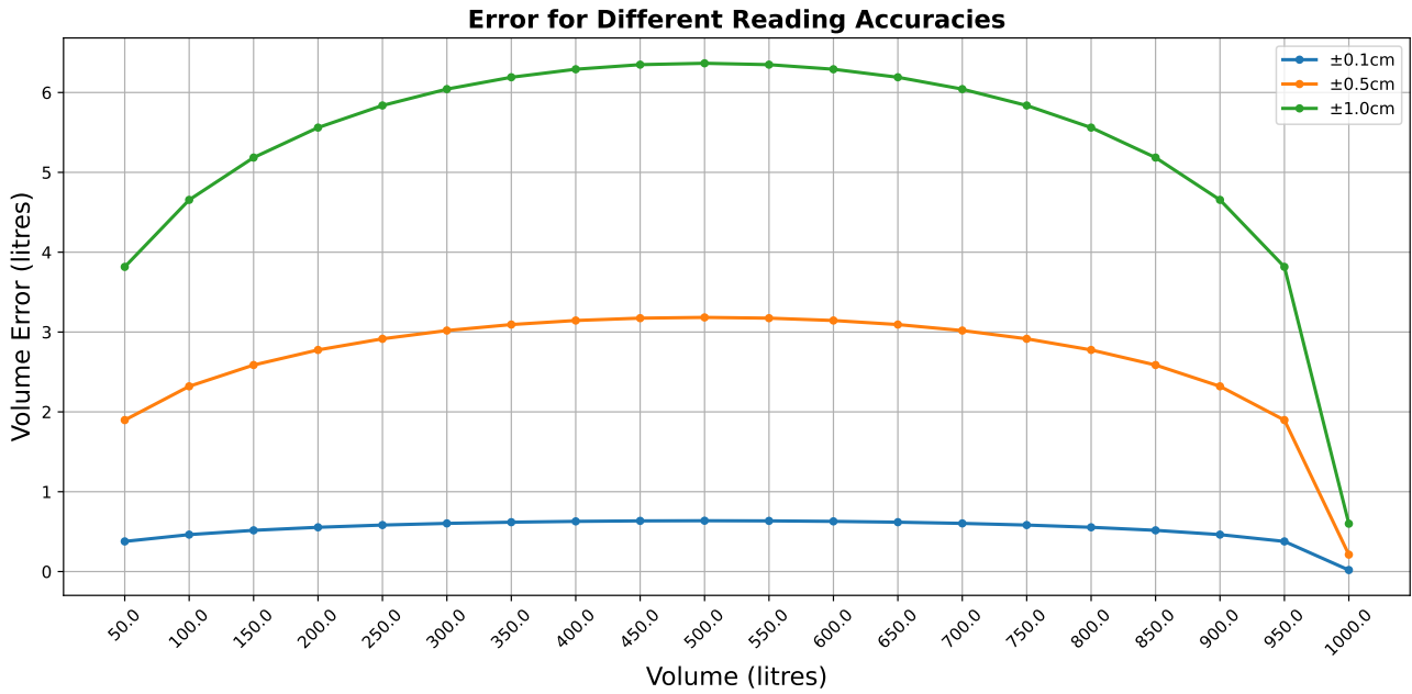
Figure 1: Absolute volume error versus fill level for three levels of dipstick reading uncertainty \pm 0.1\text{cm} (blue), \pm 0.5\text{cm} (orange) and \pm 1.0\text{cm} (green).
