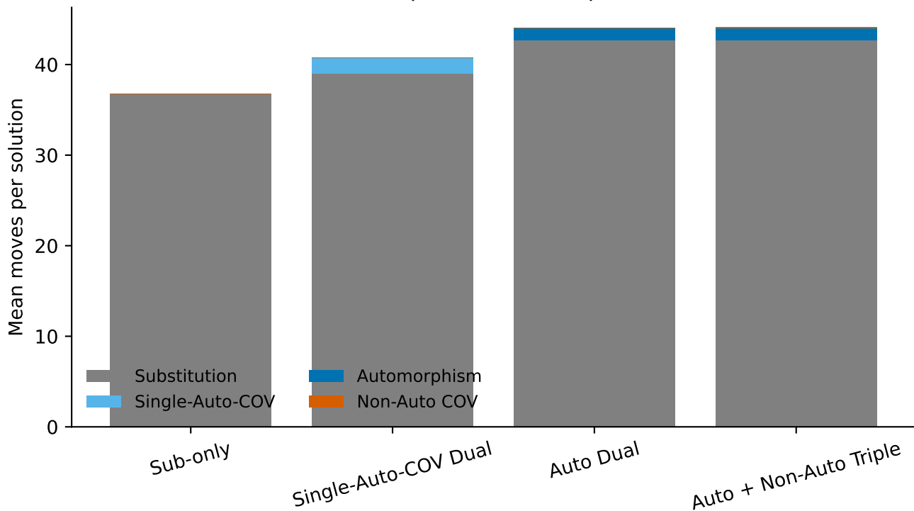
Solution-path move composition
