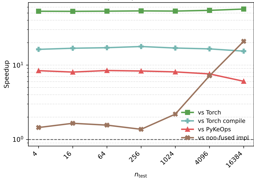
Flash Speedup (baseline / flash)
