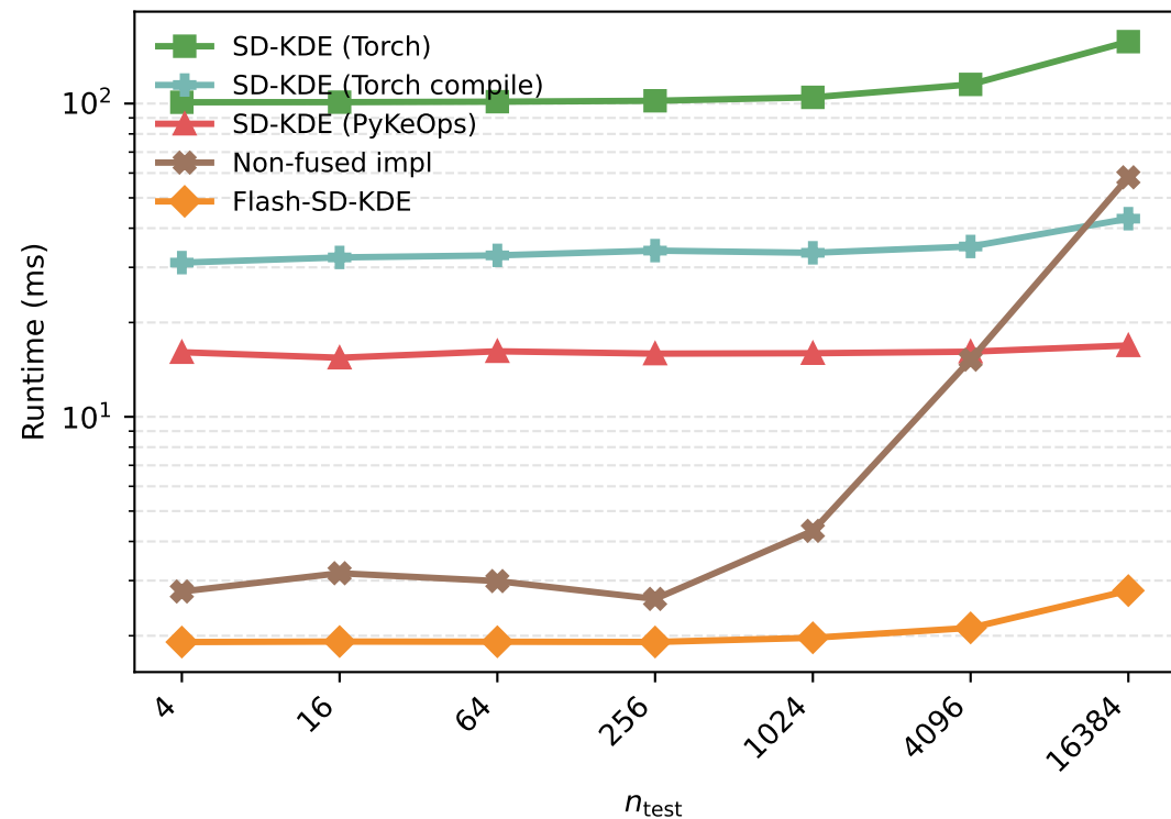
Absolute Runtime
