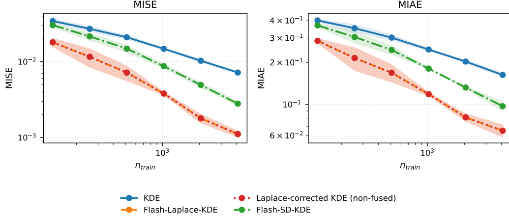
Figure 3: Oracle error on a 1D mixture-of-Gaussians benchmark. We report MISE and MIAE versus n_{train} for KDE, Flash-Laplace-KDE (fused Laplace correction), non-fused Laplace correction, and Flash-SD-KDE. The Laplace-corrected estimators can be slightly negative, so error is computed on the signed density.
