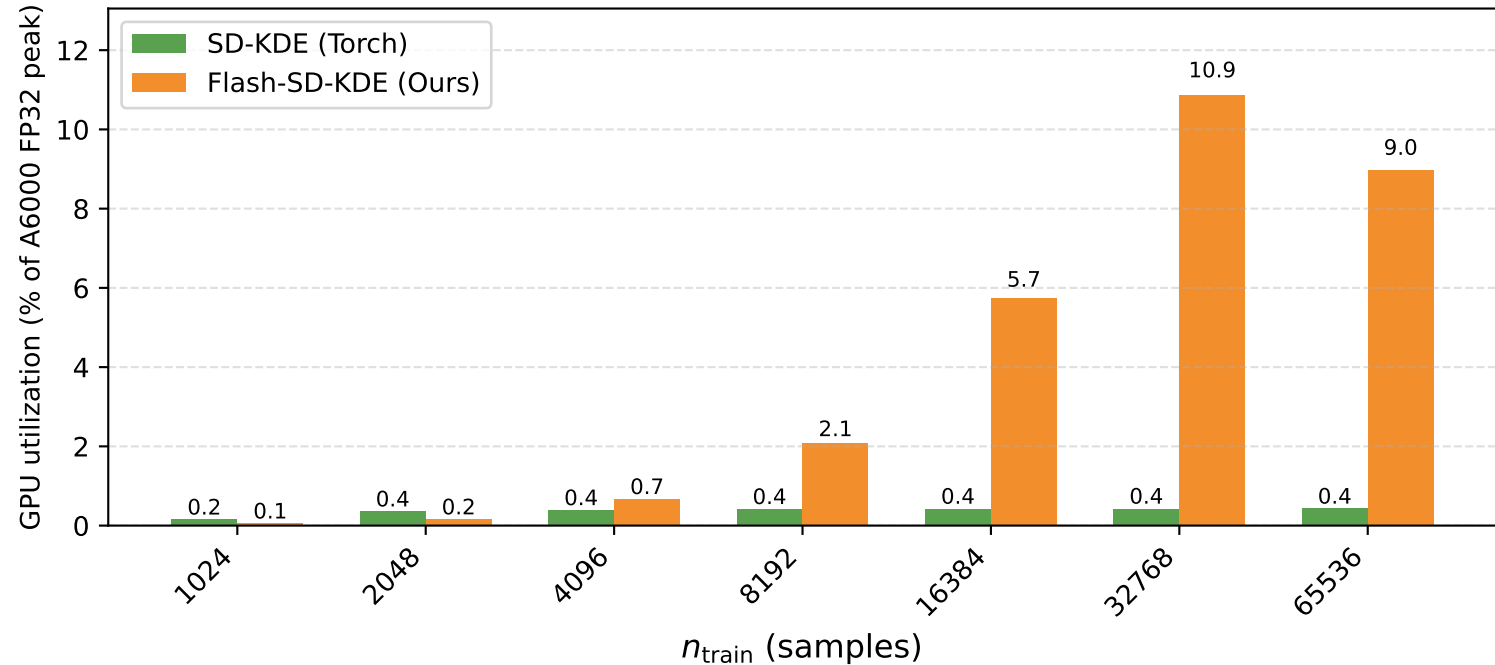
1-D SD-KDE GPU Utilization (Torch vs Flash-SD-KDE)
