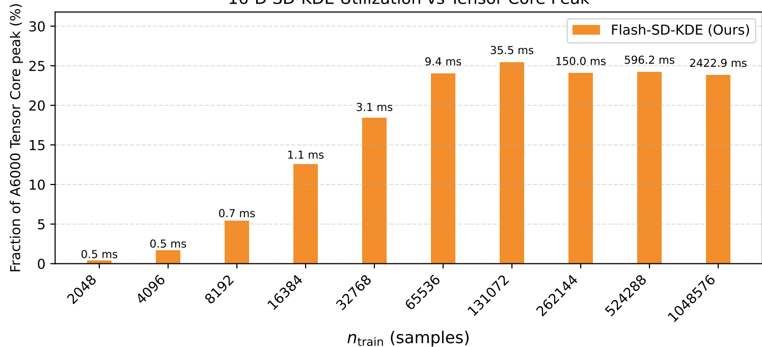
16-D SD-KDE Utilization vs Tensor Core Peak
