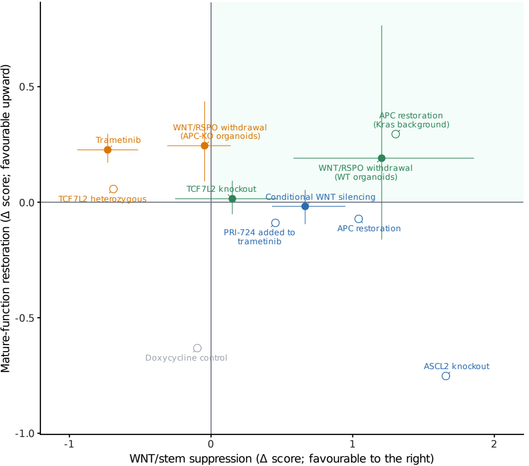
a Existing perturbations separate two response dimensions Upper right indicates simultaneous WNT/stem suppression and mature-function restoration
