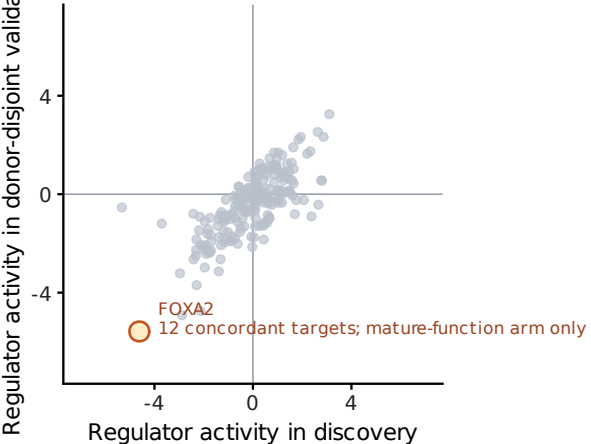
b Regulator inference yields no balanced two-arm target 201 regulators tested, one replicated regulon (Spearman \rho = 0.75 )
