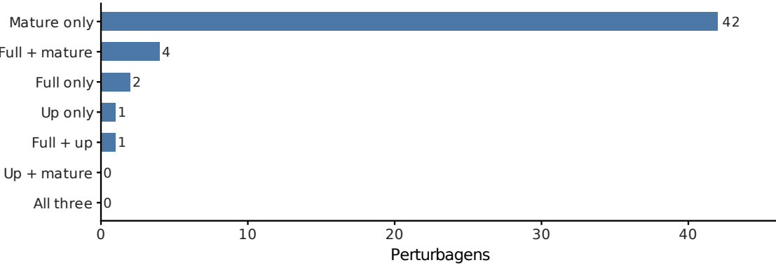
c A generic perturbation screen finds no recurrent dual-arm hit 95 opposite perturbagens returned by L1000FWD; q \leq 0.10 within each query
