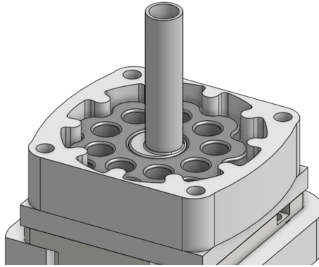
Figure 12: Input adapter seated through the cycloidal disc.
