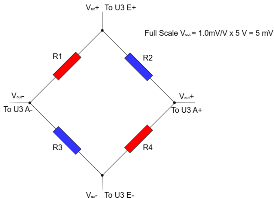
Figure 15: Full Wheatstone bridge inside LC1. R1 and R4 are in tension (resistance increases under load); R2 and R3 are in compression (resistance decreases). The differential output V_{\text{out}} is linear with applied force and self-compensating for ambient temperature changes.
