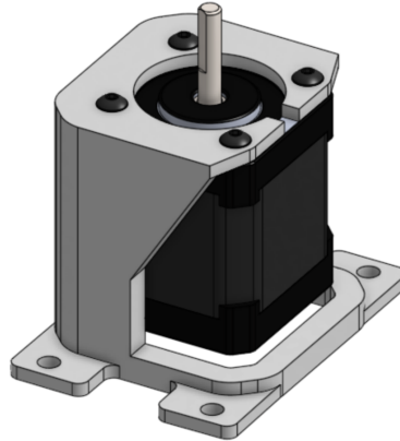
Figure 6: Auger motor mount, alternate angle showing bolt placement.
