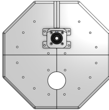
Figure 21: Auger motor assembly aligned onto the base plate.
