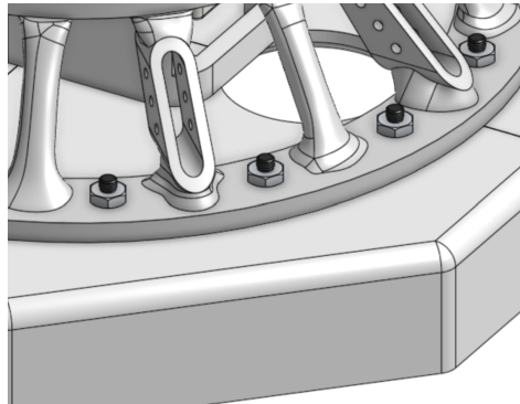
Figure 46: Support arms aligned into the base plate's mounting points.
