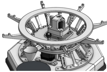
Figure 51: Support arms and funnel inserted into the trunk's slots.
