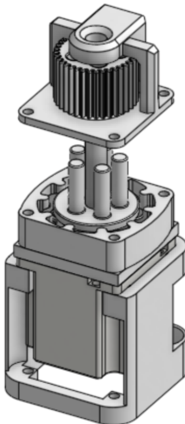
Figure 16: Exploded view of the carousel drive gear over the assembled gearbox.
