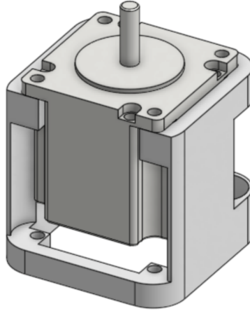
Figure 8: Carousel motor aligned with the Carousel Motor Mount.
