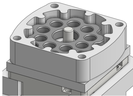
Figure 11: Cycloidal disc lowered into the housing with the input adapter engaging the motor shaft.
