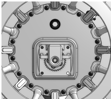
Figure 50: Bolts and nuts inserted through the trunk's aligned mounting holes.
