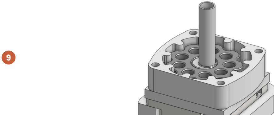
Figure 12: Input adapter seated through the cycloidal disc.
