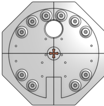
Figure 20: Dovetail key inserted at the center junction of the four base quadrants.
