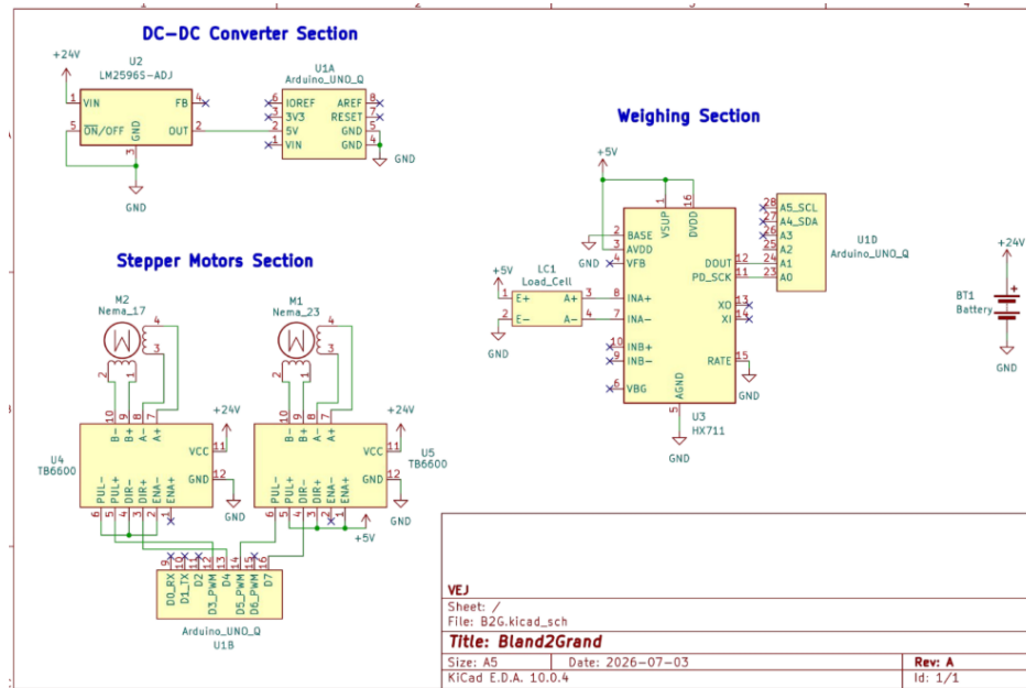
Figure 56: Full electrical schematic for Bland2Grand, covering the controller, stepper drivers, motors, and load cell.
