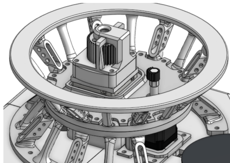
Figure 49: Upper and lower trunk sections joined together.
