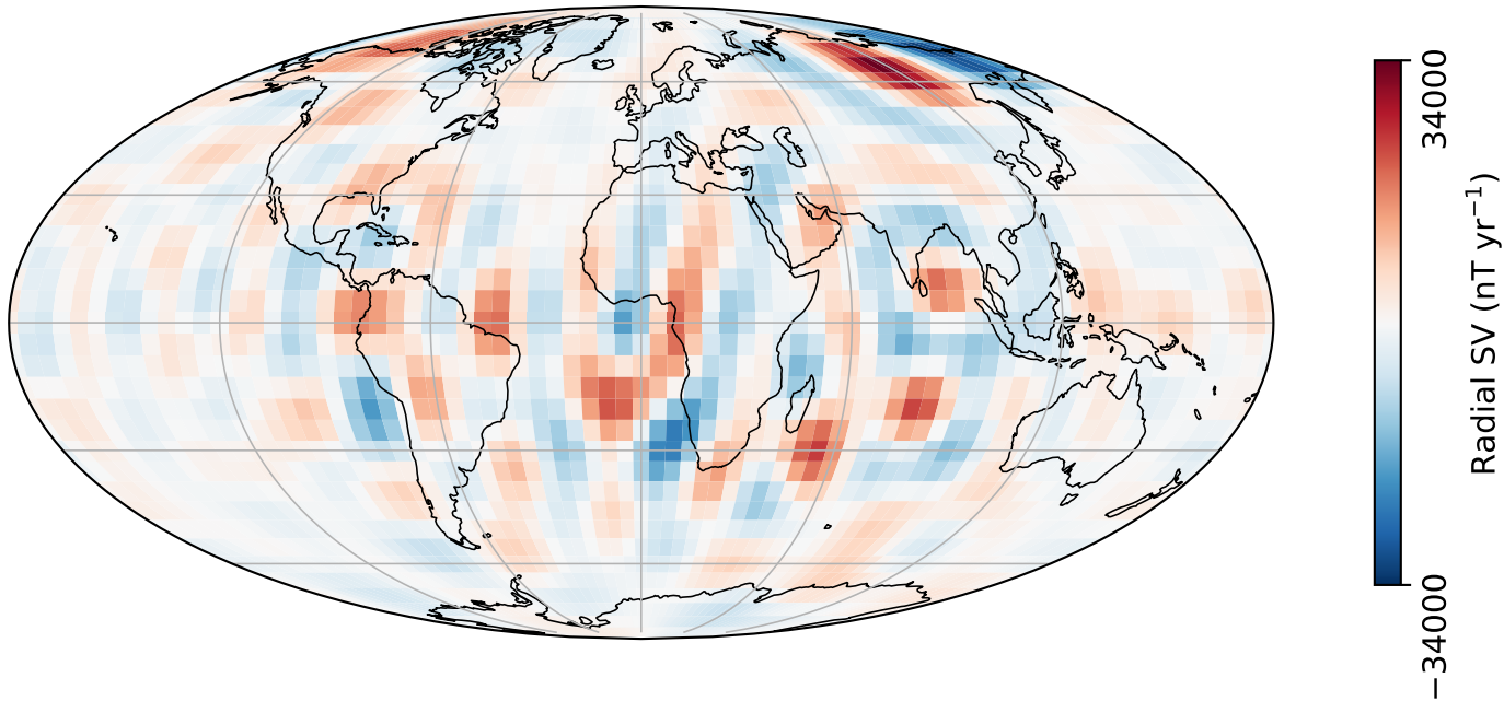
CHAOS-8.6 radial SV at 2015.0 at the CMB ( r = 3485 (km))
