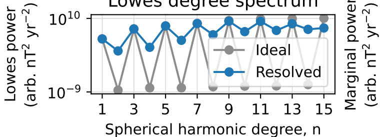
Lowes degree spectrum
