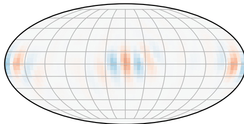
Resolved radial SV
