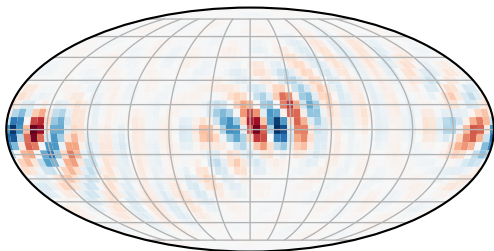
Ideal radial SV
