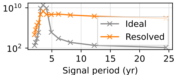
Period spectrum ( n \leq 15 )
