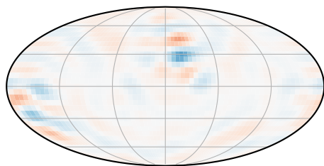
Scaled resolved modes
