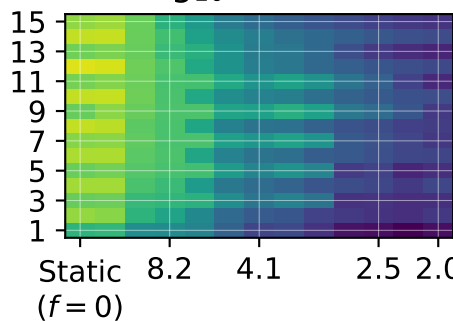
Scaled resolved modes RMS \log_{10} misfit = 1.84
