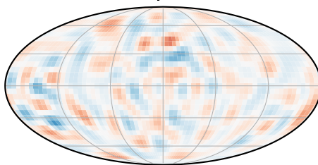
Modes + spectral infill
