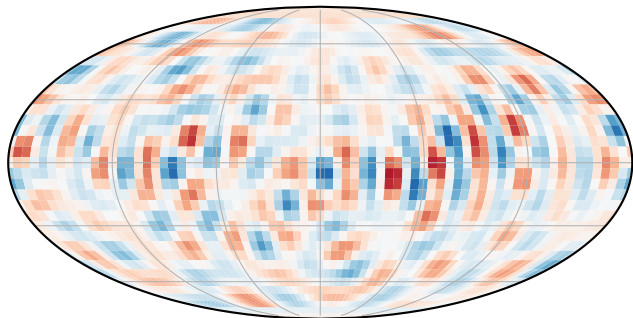
Perturbation 1 radial SV Year 2015.0
