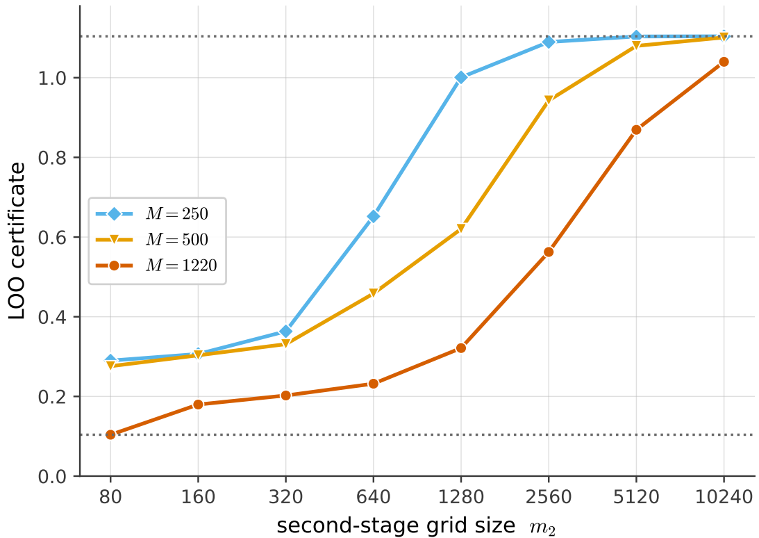
C2 transductive leave-one-out certificate (Thm 4.9): the vacuity slide toward \alpha + B 8B operating bag M = 1,220
