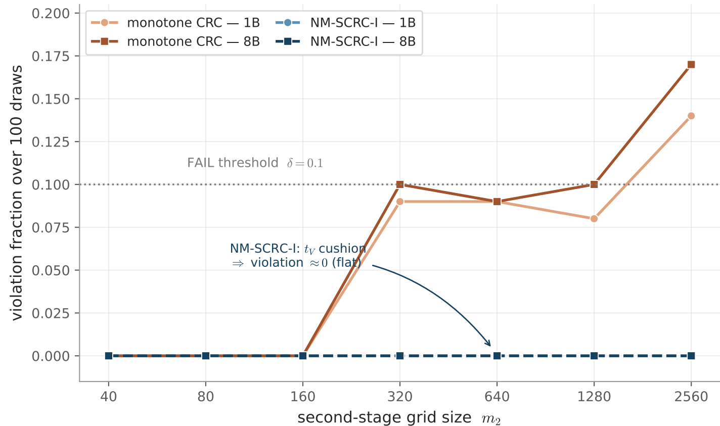
Violation fraction vs grid size m_2 : monotone CRC (1B, 8B) vs NM-SCRC-I
