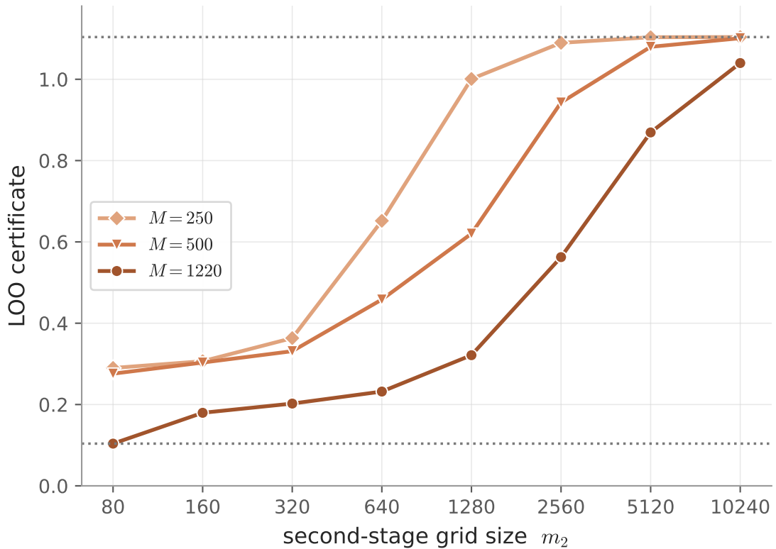
C2 transductive leave-one-out certificate (Thm 4.9): the vacuity slide toward \alpha + B 8B operating bag M = 1,220 Onset shifts right as M grows
