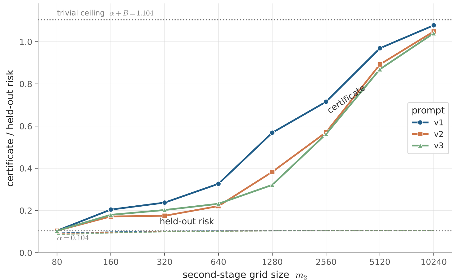
C2 certificate across prompts (8B, M=1,220 )
